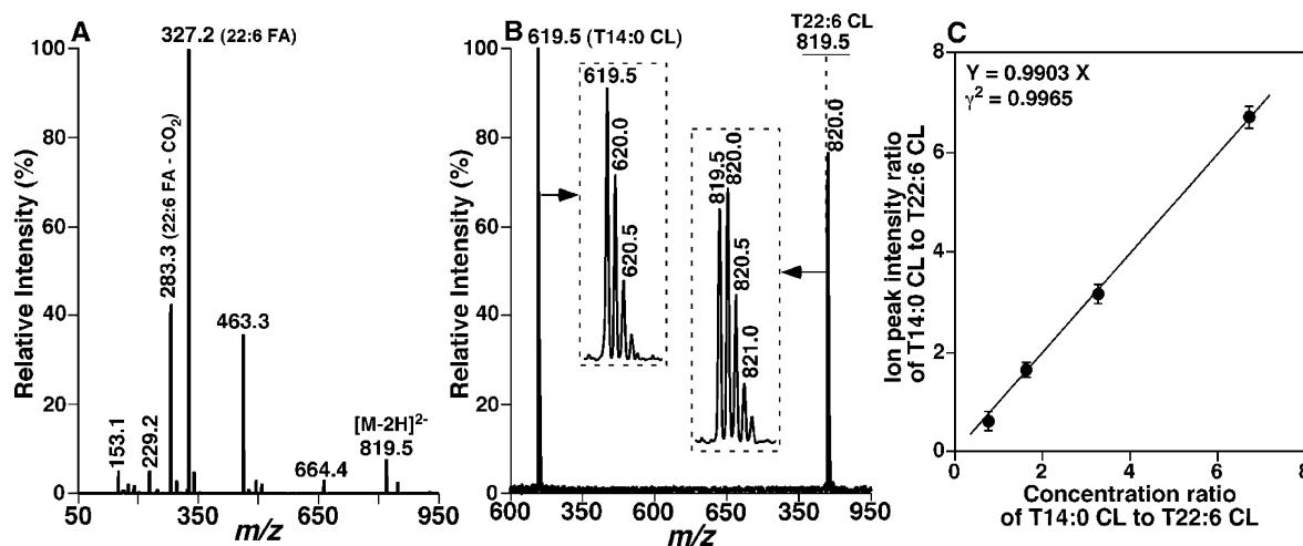
FIGURE 2: Electrospray ionization mass spectrometric analyses of synthesized tetra22:6 cardiolipin. (A) Product ion mass spectrum of m/z 819.5, from which the selected ion can be identified as T22:6 CL. (B) Representative negative-ion ESI mass spectrum of an equimolar mixture of T14:0 CL and T22:6 CL (1 pmol/ \mu L each). The insets display the isotopologue patterns of the ions. The horizontal line over the ion peak at m/z 819.5 represents the monoisotopic ion peak intensity after ^{13}\text{C} de-isotoping and has been normalized to that at m/z 619.5. (C) Linear correlation between the concentration ratios and the ion peak intensity ratios of T14:0 CL and T22:6 CL. The data points represent the mean \pm SD determined at a variety of concentrations. These results indicate that the ionization response factors of T14:0 CL and T22:6 are essentially identical within experimental errors after ^{13}\text{C} de-isotoping.
