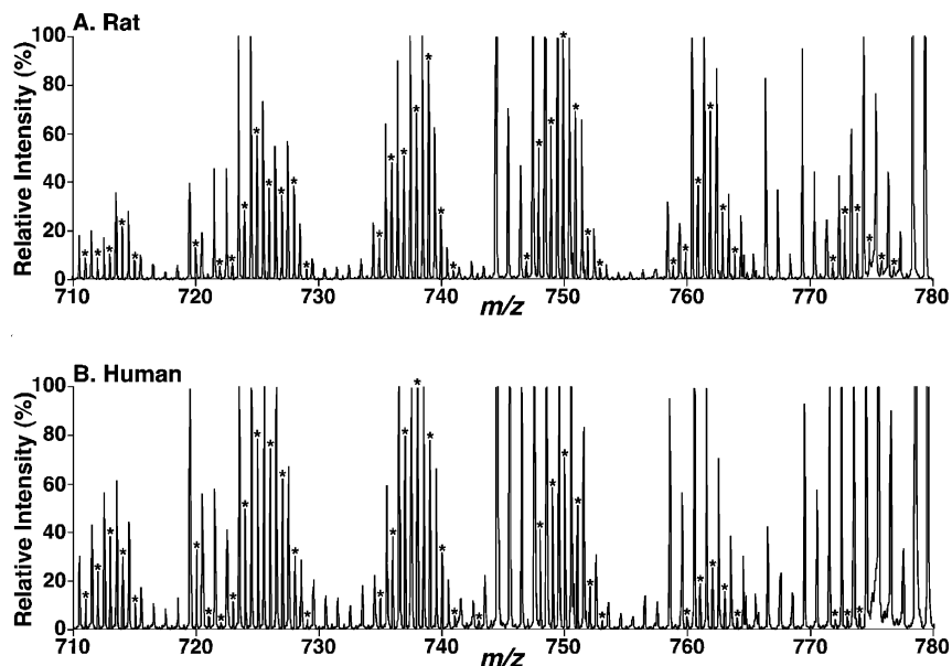
FIGURE 3: Expanded representative negative-ion ESI mass spectra of lipid extracts of rat and human brain samples using a QqTOF mass spectrometer. Lipid extracts of rat cortex (A) and human cortex (B) were prepared by a modified Bligh and Dyer procedure, and electrospray ionization mass spectra were acquired in the negative-ion mode using a QqTOF mass spectrometer as described under the Materials and Methods. The asterisks indicate the identified CL plus-one isotopologues, which were characteristic of doubly charged CL molecular species and were used to quantify individual CL molecular species based on ion intensity as previously described (10). Each spectrum is displayed after being normalized to the most abundant CL plus-one isotopologue.
