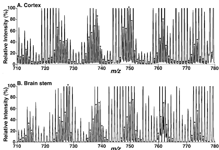
FIGURE 1: Expanded negative-ion ESI mass spectra of mouse brain lipid extracts obtained using a QqTOF mass spectrometer. Lipid extracts of mouse cortex (A) and brain stem (B) were prepared by a modified Bligh and Dyer procedure, and electrospray ionization mass spectra were acquired in the negative-ion mode using a QqTOF mass spectrometer as described under the Materials and Methods. The asterisks indicate the identified CL plus-one isotopologues, which were characteristic of the doubly charged CL molecular species and were used to quantify individual CL molecular species based on ion intensity as previously described (10). Each spectrum is displayed after being normalized to the most abundant CL plus-one isotopologue.
