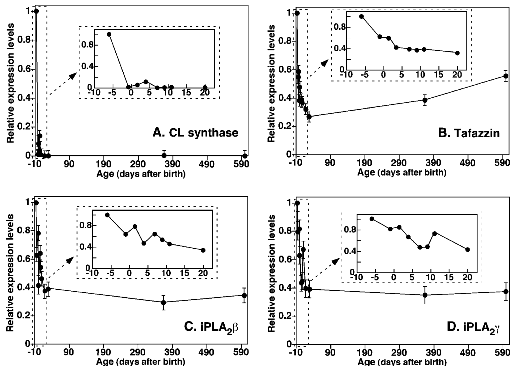
FIGURE 6: Temporal changes of the relative mRNA levels of select CL biosynthetic and remodeling enzymes in mouse cortex before and after birth using quantitative real-time PCR analyses. Total RNA was isolated, and quantitative PCR was performed as described under the Materials and Methods. The forward and reverse primers as well as probes for CL synthase (A), tafazzin (B), calcium-independent phospholipase A 2 \beta (iPLA 2 \beta ) (C) and iPLA 2 \gamma (D) used in the analyses are listed under the Materials and Methods. Data represent the mean \pm SD from separate preparations and analyses of at least three different animals. Data are expressed as normalized arbitrary units, with message levels normalized to that of mouse GAPDH, which was used as an internal control. The inset of each panel expands the pre- and postnatal time period.
