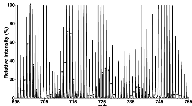
FIGURE 8: Expanded negative-ion ESI mass spectrum of lipid extracts of primary neuronal cultures using a QqTOF mass spectrometer. Lipid extracts of cultured cells were prepared by a modified Bligh and Dyer procedure, and an ESI mass spectrum was acquired in the negative-ion mode using a QqTOF mass spectrometer as described under the Materials and Methods. The asterisks indicate the recognizable CL plus-one isotopologues, which were characteristic of doubly charged CL molecular species and were used to quantify individual CL molecular species based on ion intensity as previously described (10). The spectrum is displayed after being normalized to the most abundant CL plus-one isotopologue.
